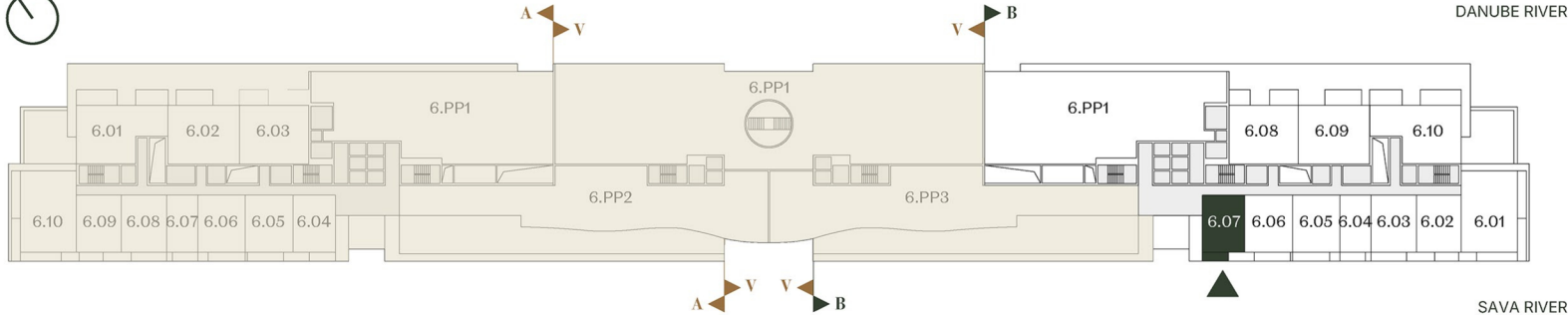
LEVEL PLAN
